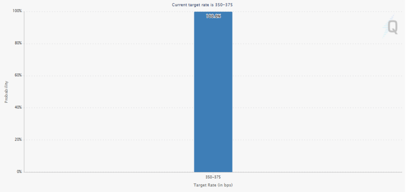
Target Rate Probabilities for 29 Apr 2026 Fed Meeting
